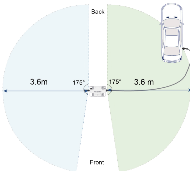
Figure 2-5 Actual working radius of the 5-meter cable
