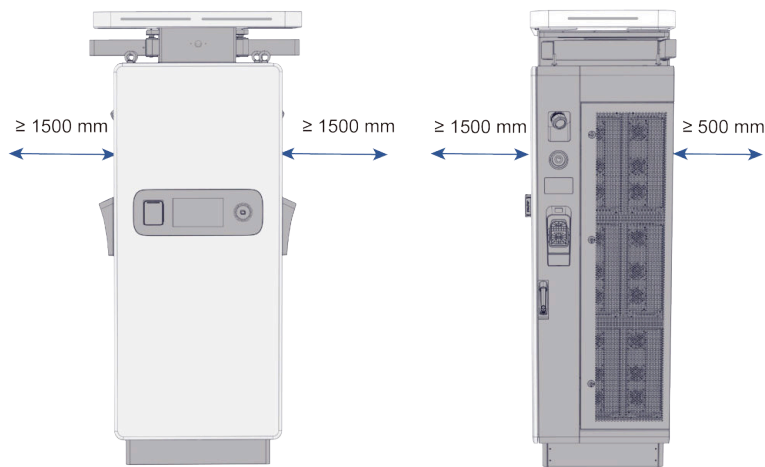
Figure 3-1 Space Requirements for Installation
