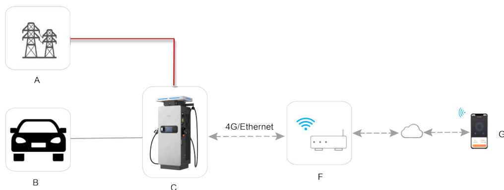
Figure 2-3 Remote Charging
